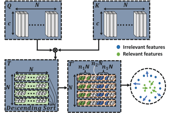
Figure 4: The illustration of our contrastive learning scheme for ENLCA. For each ordered sequence, we take the top n_1 N related ones as relevant features and n_1 N unrelated ones starting from n_2 N as irrelevant features.
