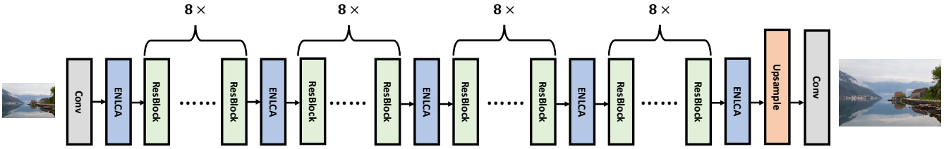
Figure 3: The proposed Efficient Non-Local Contrastive Network (ENLCN). Five ENLCA modules are embedded after every eight residual blocks.
