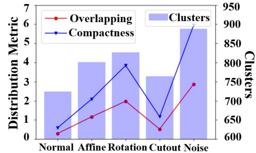
Figure 4: We show the distribution overlapping and distribution dispersity related with clusters of different augmentations.
