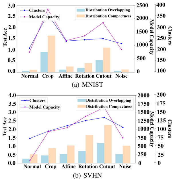
Figure 5: Experimental results on MNIST and SVHN datasets. We use the number of clusters, decision tree nodes to measure sample complexity and model capacity.
