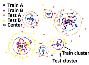
Figure 1: We conduct a simple validation to fit the points of two classes (A and B) in the left graph using SVM classifier with default settings. We respectively fit the central point of each cluster(blue point) and the complete training set (blue and purple points). The variance of clusters in test set is set as two times of that in train set. The size of dotted circle represents the size of clusters.
