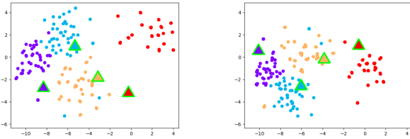
Figure 8: t-SNE feature embedding of query videos ( circles ) and support prototypes ( triangles ) on HMDB. Left/Right: before/after applying our alignment.
