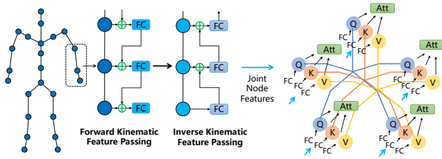
Figure 3: The Kinematic Propagation Module (KPM) and the Structured Multi-head Attention. Features are embedded and passed along the kinematic chains forward and inversely with fusion operations. Note that the endpoints of feature passing are root and leaf nodes, and we just show a part of them for clearer view.
