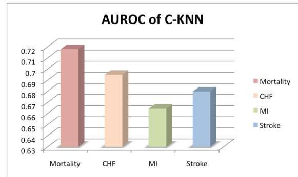
Figure 2: AUROC of C-KNN
