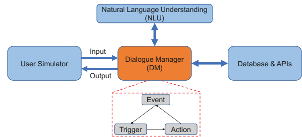
Figure 1: The architecture of Carina Dialog System
