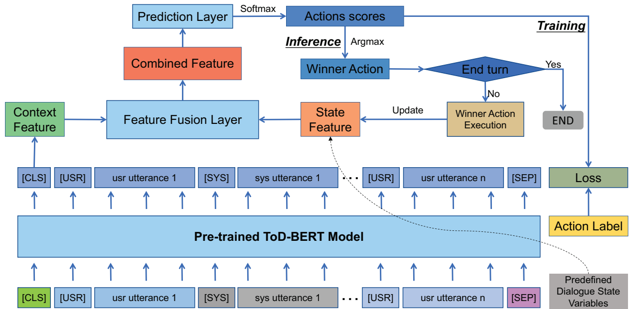
Figure 2: The architecture of Model-Trigger DM
