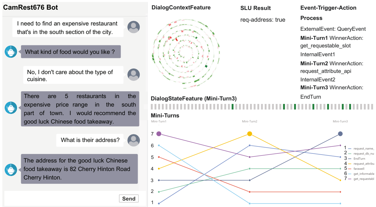
Figure 3: Demo showing the process of Model-Trigger DM.
