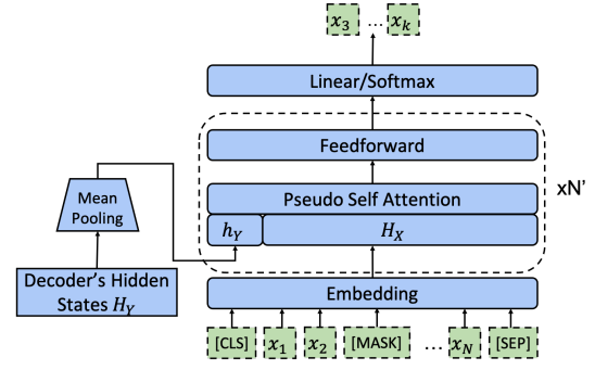
Figure 3: The overview of the claim reconstructor. It is also the PSA structure where we inject the mean pooling of decoder’s hidden states to its key-value pairs. N' is the number of PSA blocks.
