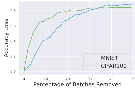
Figure 7: Test accuracy on all classes with increased amnesiac unlearning (mean of 10 runs)
