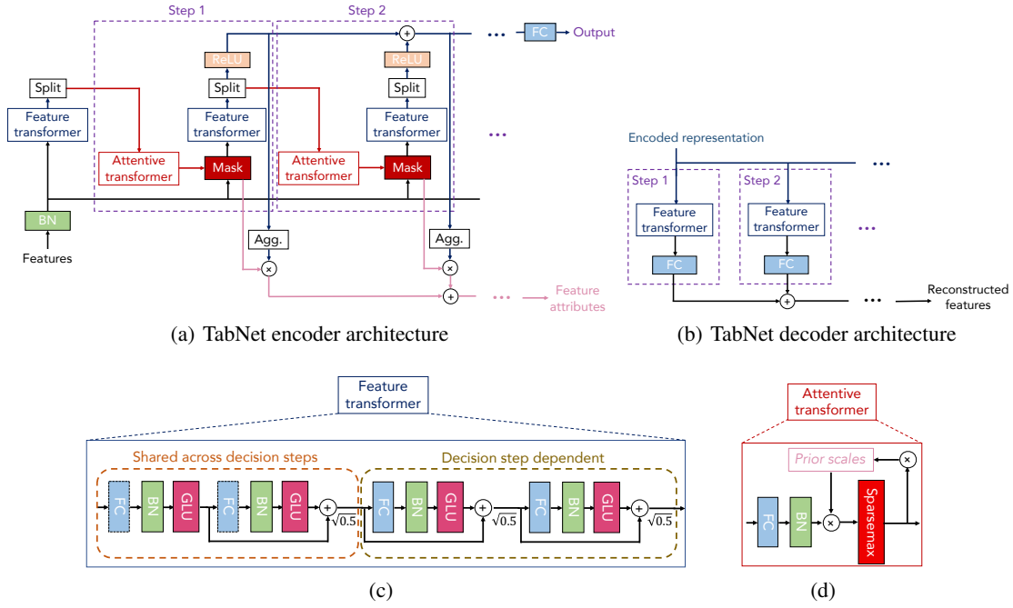
Figure 4: (a) TabNet encoder, composed of a feature transformer, an attentive transformer and feature masking. A split block divides the processed representation to be used by the attentive transformer of the subsequent step as well as for the overall output. For each step, the feature selection mask provides interpretable information about the model’s functionality, and the masks can be aggregated to obtain global feature important attribution. (b) TabNet decoder, composed of a feature transformer block at each step. (c) A feature transformer block example – 4-layer network is shown, where 2 are shared across all decision steps and 2 are decision step-dependent. Each layer is composed of a fully-connected (FC) layer, BN and GLU nonlinearity. (d) An attentive transformer block example – a single layer mapping is modulated with a prior scale information which aggregates how much each feature has been used before the current decision step. sparsemax (Martins and Astudillo 2016) is used for normalization of the coefficients, resulting in sparse selection of the salient features.
