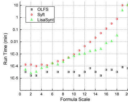
Figure 3: Results on the pattern formula GF(n) = \square p_1 \wedge (\bigwedge_{i=2..n} \diamond p_i) .
