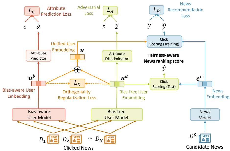
Figure 2: The architecture of our FairRec approach.
