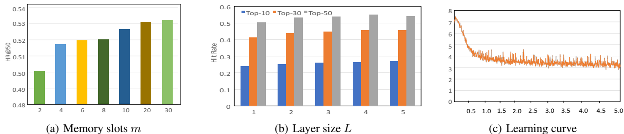
Figure 2: The proposed DMAN analysis
