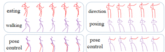
Figure 6: Fine-grained control over different chains in the predicted motion. In the left figure, we predict a ‘walking’ action (purple) with the right leg following the action of ‘eating’ (red). The result is shown on the bottom row with matching colors. In the right figure, we predict a ‘posing’ action with the left hand following the ‘direction’ action.
