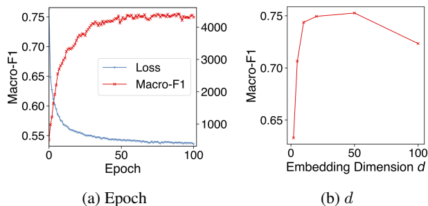
Figure 3: Parameter analysis for sign prediction.
