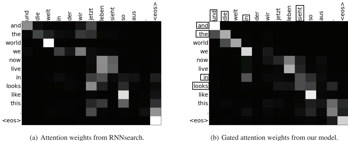
Figure 2: Visualization of the attention weights for one De-En translation case. The x-axis and y-axis of each plot correspond to the words in the source sentence (German) and the target sentence (English). 2(a) is attention weights from RNNsearch, 2(b) is gated attention weights from our model. The different and important parts are emphasized with rectangle.
