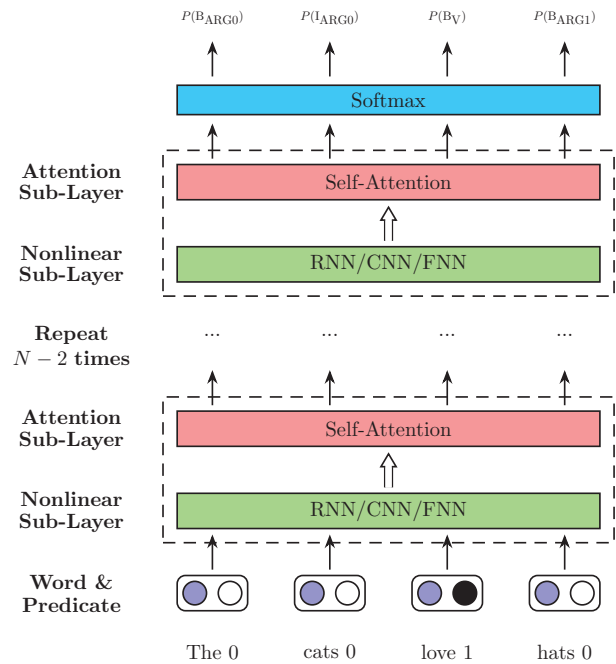
Figure 1: An illustration of our deep attentional neural network. Original utterances and corresponding predicate masks are taken as the only inputs for our deep model. For example, love is the predicate and marked as 1, while other words are marked as 0.
