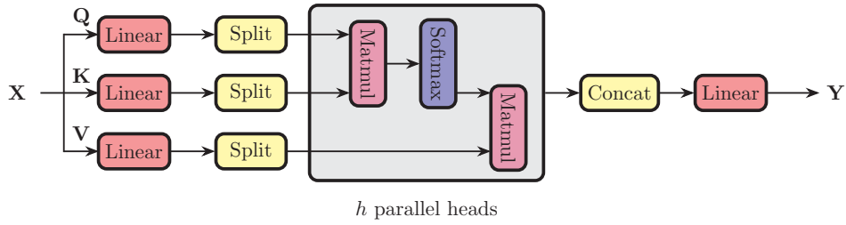
Figure 2: The computation graph of multi-head self-attention mechanism. All heads can be computed in parallel using highly optimized matrix multiplication codes.
