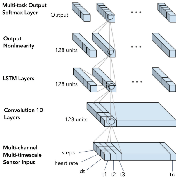
Figure 2: DeepHeart architecture.
