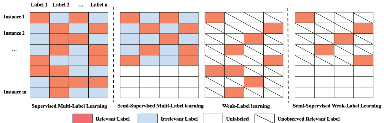
Figure 1: Four multi-label learning settings
