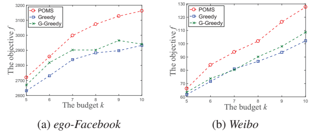
Figure 2: Generalized influence maximization.
