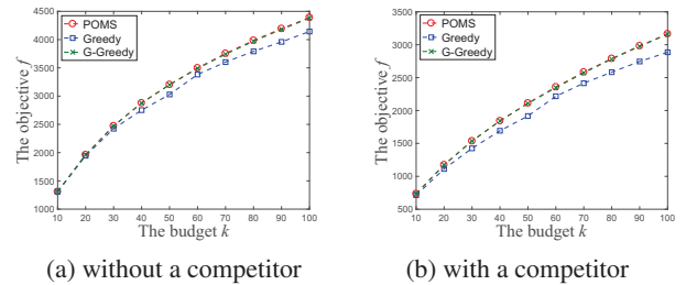
Figure 1: Budget allocation on the Yahoo! data set.
