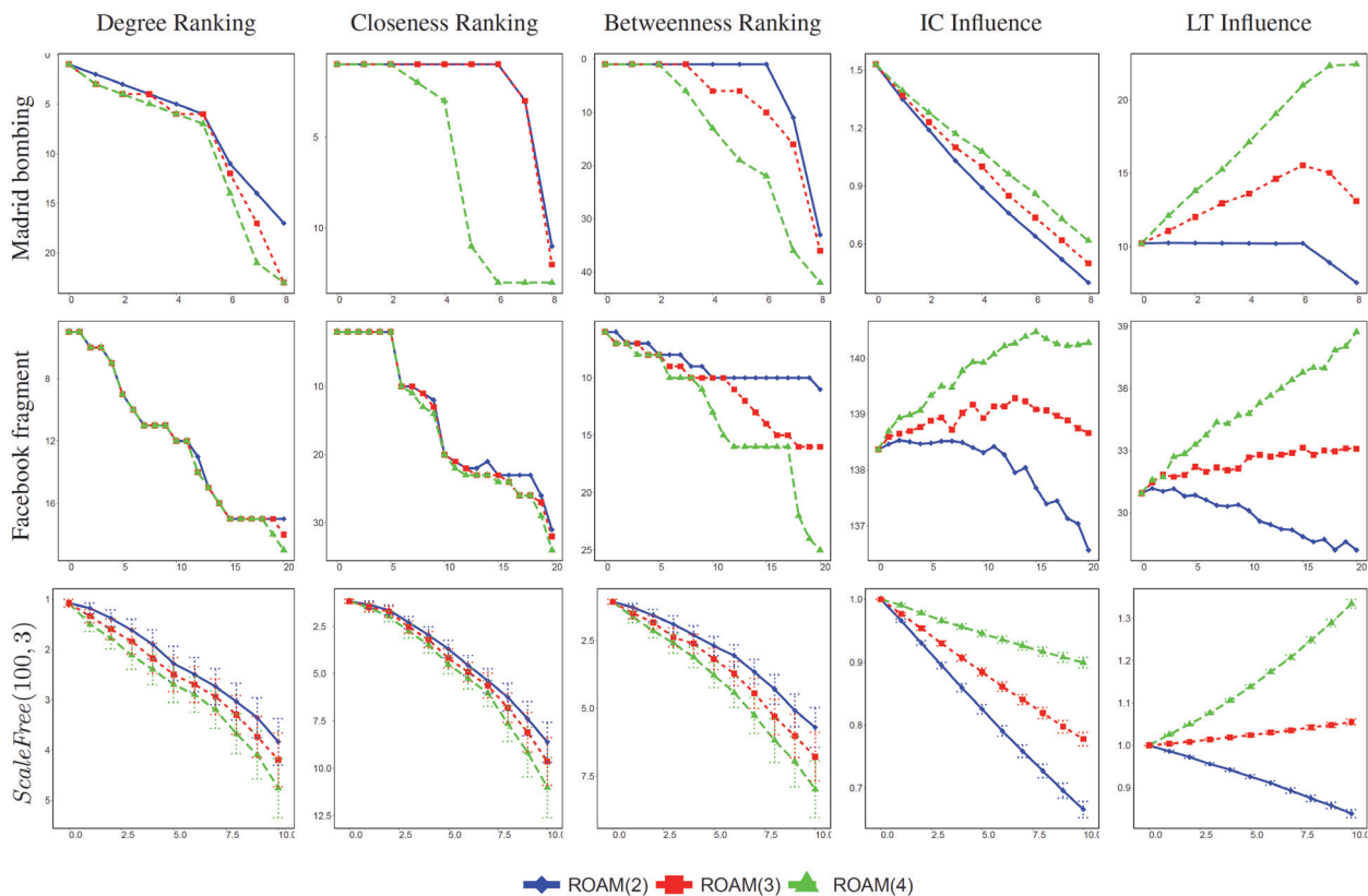
Figure 2: (Figure 3 from Waniek et al, 2016a) Executing ROAM multiple, consecutive times, where the x -axis represents the number of executions. The subfigures show the source node’s ranking (according to different centrality measures), and the relative change in its influence value (according to different influence models) for the Madrid-attack network, 50 scale-free networks, and a medium-sized fragment of Facebook’s network (333 nodes, 5038 edges). The size of the budget b is 2, 3, or 4.
