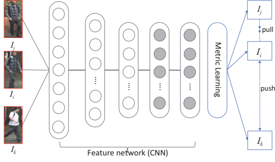
Figure 2: Illustration of our learning formulation. It tends to maximize the distance disparity between the matched pair and mismatched pair for each triplet, in terms of optimization.
