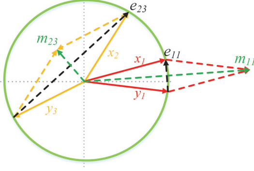
Figure 1: An illustration of difference and commonness in 2-dimensional Euclidean space. Each feature is l_2 -normalized. (x_1, y_1) (red) denotes a similar pair while (x_2, y_3) (yellow) represents a dissimilar pair. The green circle is a unit one.
