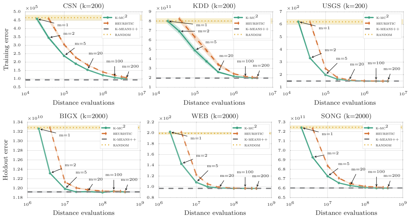
Figure 1: Average quantization error vs. number of distance evaluations for K-MC 2 and HEURISTIC as well as the average quantization error (without the number of distance evaluations) for k-means++ and RANDOM. K-MC 2 quickly converges to full k-means++ and outperforms HEURISTIC. Shaded areas denote 95% confidence intervals.
