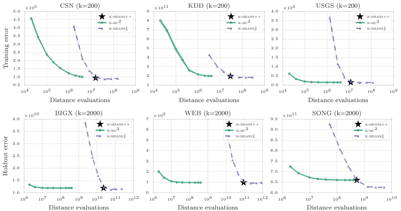
Figure 2: Average quantization error vs. number of distance evaluations for K-MC 2 , k-means++ and k-means||. K-MC 2 obtains competitive solutions significantly faster than both k-means++ and k-means||.
