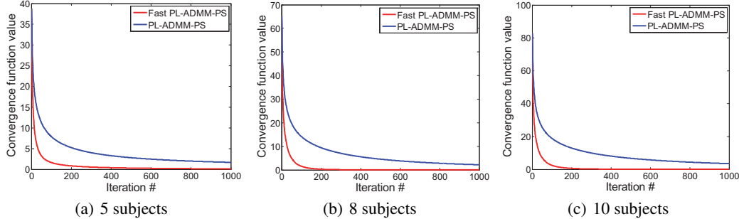
Figure 3: Plots of the convergence function values of (16) in each iterations by using PL-ADMM-PS and Fast PL-ADMM-PS for (24) with different sizes of data \mathbf{X} for subspace clustering.
