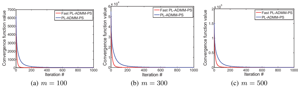
Figure 2: Plots of the convergence function values of (16) in each iterations by using PL-ADMM-PS and Fast PL-ADMM-PS for (23) with different sizes of \mathbf{X} \in \mathbb{R}^{m \times m} .
